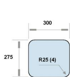
Minimum external dimensions at the section A-A
