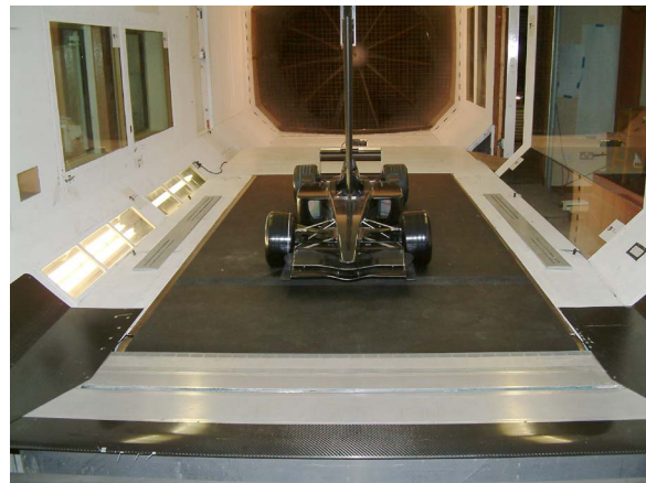
Fig. 6 Image of a race car model in a low speed wind tunnel equipped with a moving belt system
